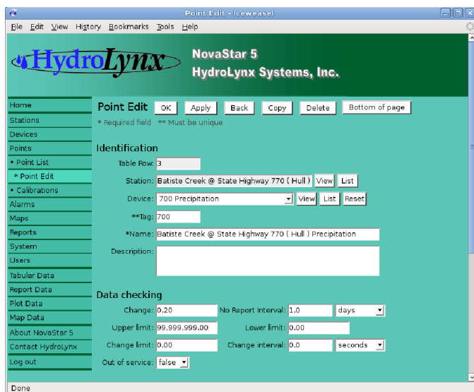
Model 5073NS-5 NovaStar5 Database setup screen
