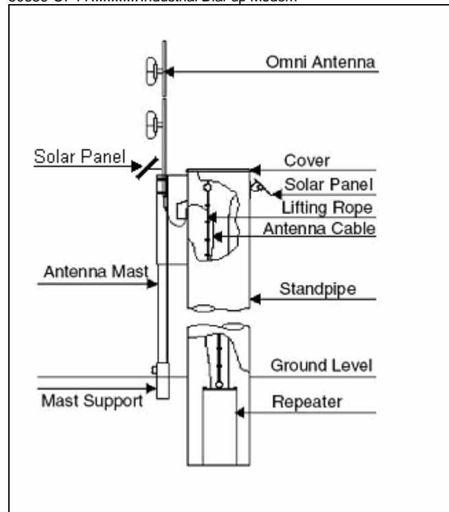
Model 50386P Packaged Repeater
