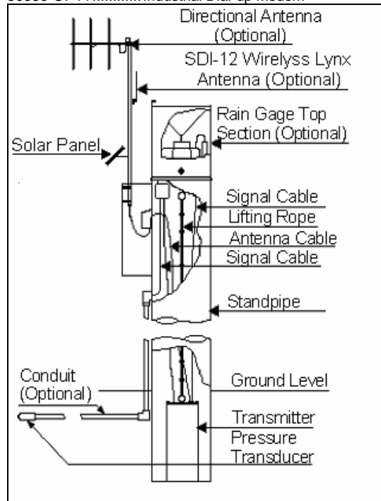
Model 5390 Packaged Pressure Transducer Station
