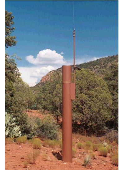
Self-Reporting Rain Station, Yavapai County, AZ
